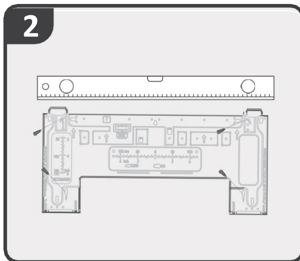
Fixez la plaque support
